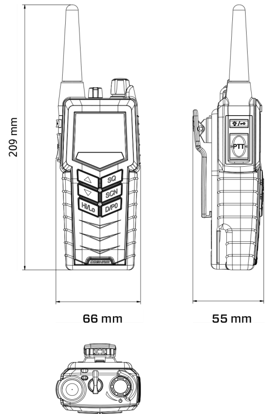
SAILOR 3965 UHF Fire Fighter
