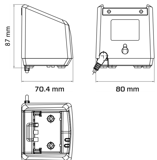
SAILOR CH 3505 Single Charger Unit
